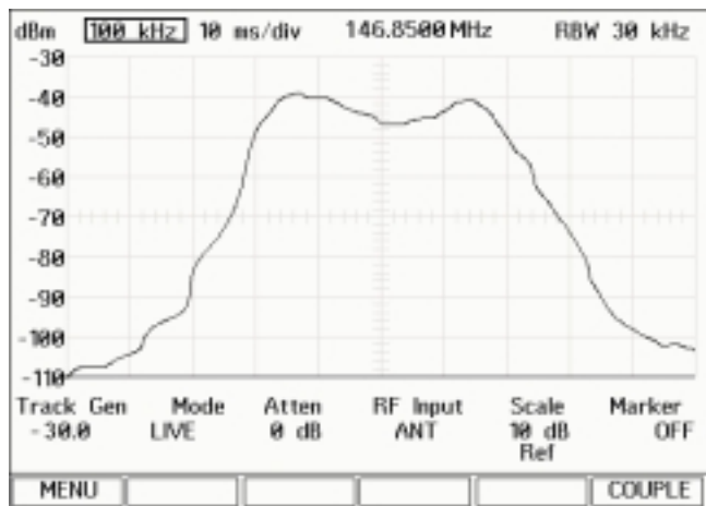
Figure 3.0 - Tuning the RF Filters on the Front End of the Receiver
