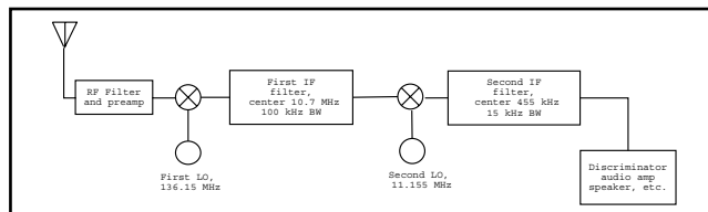
Figure 1.0 - Radio Receiver Block Diagram
