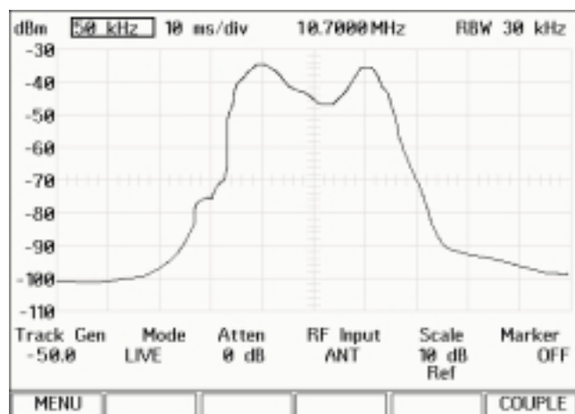
Figure 5.0 - First IF Display Indicating Alignment is Required
