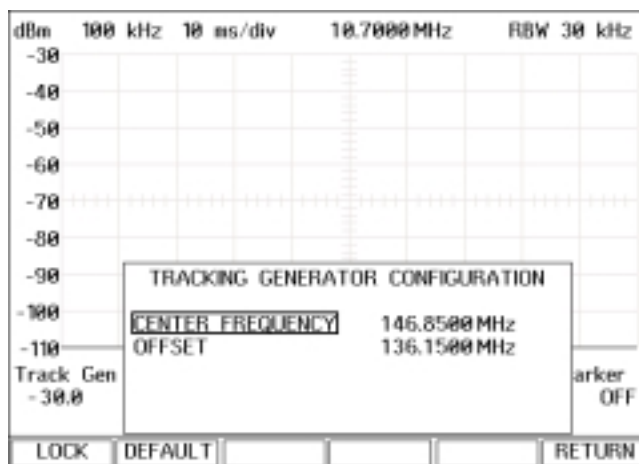
Figure 2.0 - Configuring the Tracking Generator
