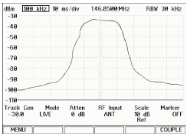
Figure 4.0 - Results of the Alignment after Adjusting the Radio's Input Filters
