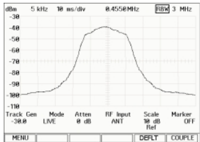
Figure 8.0 - Opening up the Resolution Bandwidth to 3 MHz
