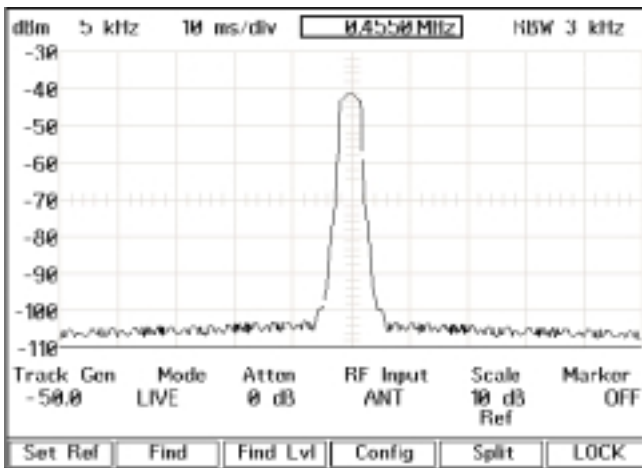
Figure 7.0 - Results of Changing the Span to 5 KHz/division
