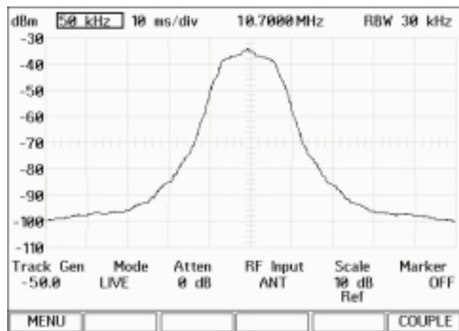
Figure 6.0 - IF After Alignment with Gain of 10 dB
